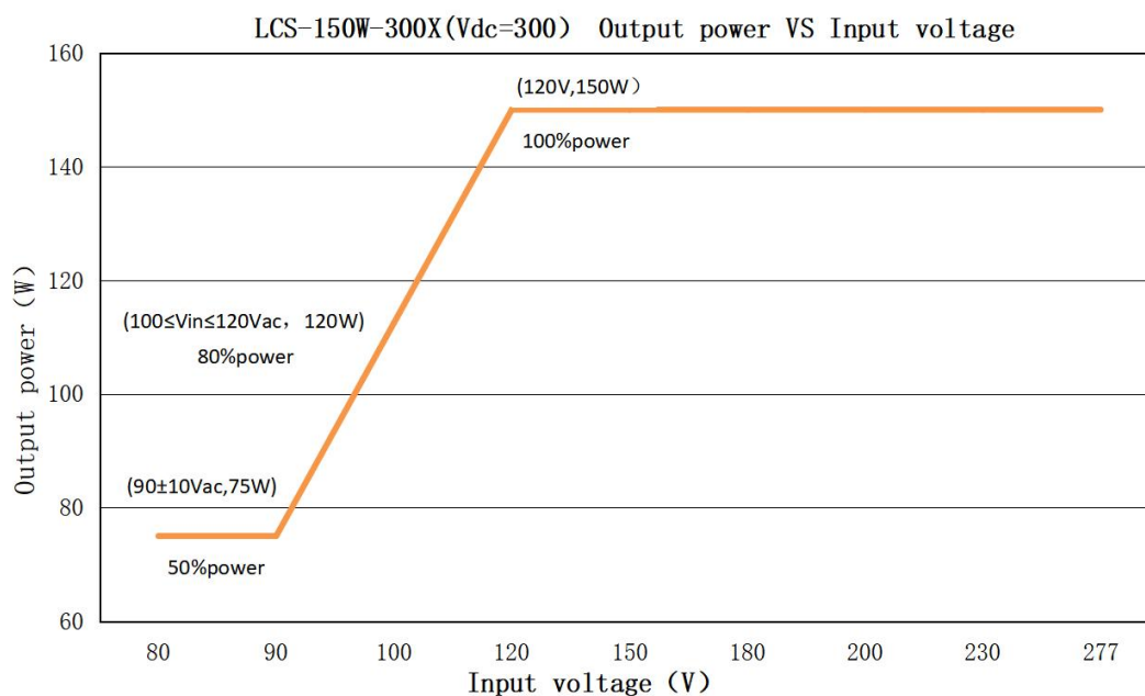
LCS-150W-300X(For output 300Vdc, the rated output current & power under different input voltage)
