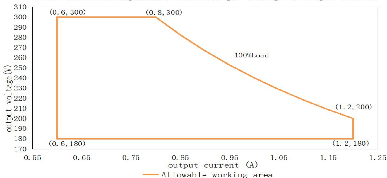
LCS-240W-300X (Import:120–277Vac) output voltage VS output current
