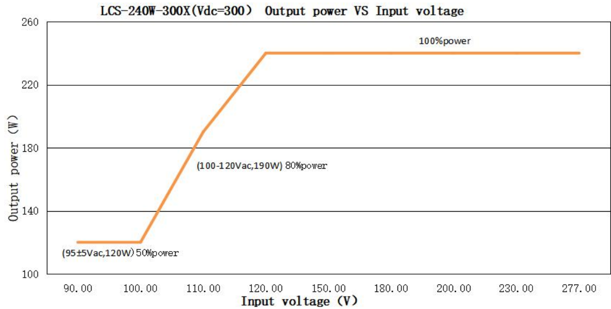
LCS-240W-300X(For output 300Vdc, the rated output current & power under different input voltage)
