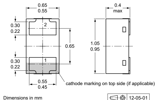
Fig. 16. Package outline DFN1006D-2 (SOD882D)
