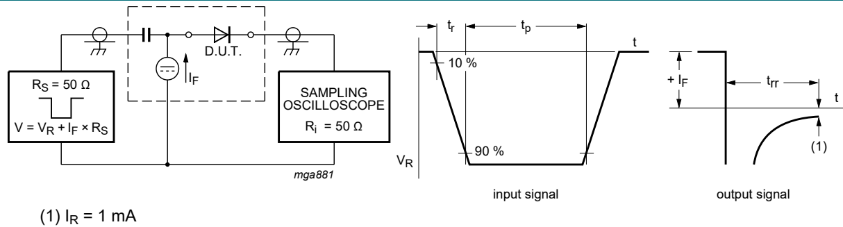
Fig. 14. Reverse recovery time: test circuit and waveforms
