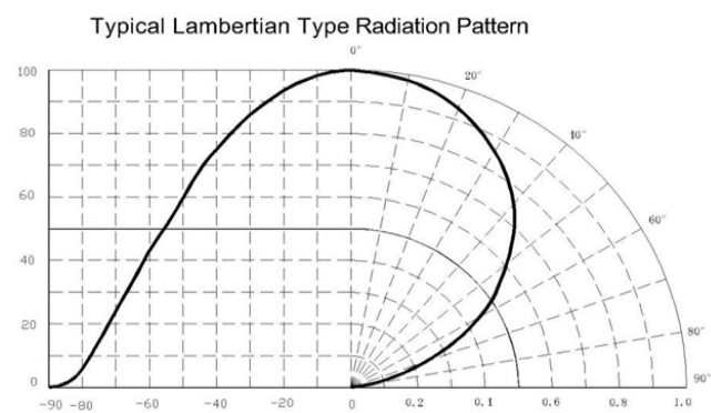
Radiation diagram
