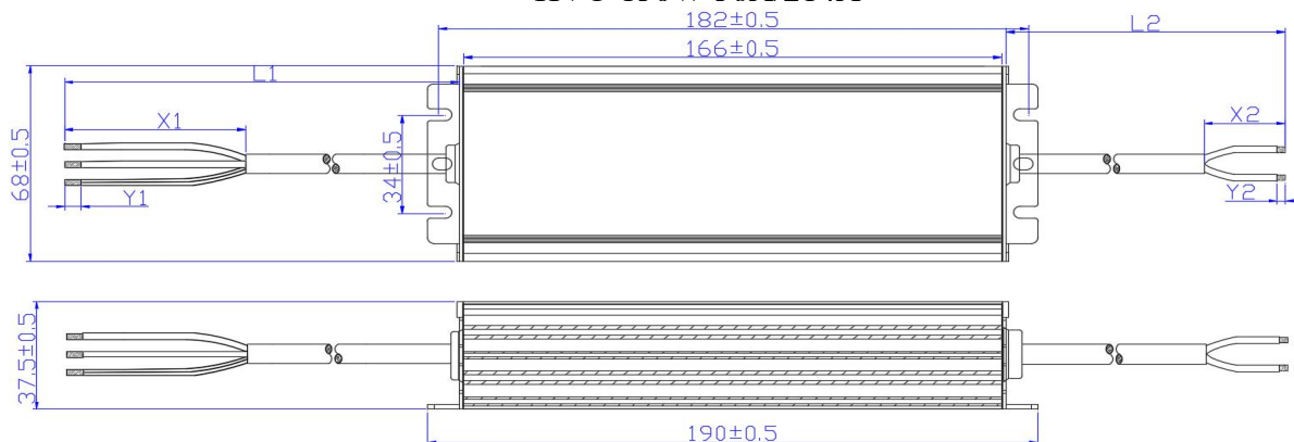
HVC-150W-56B/214B
