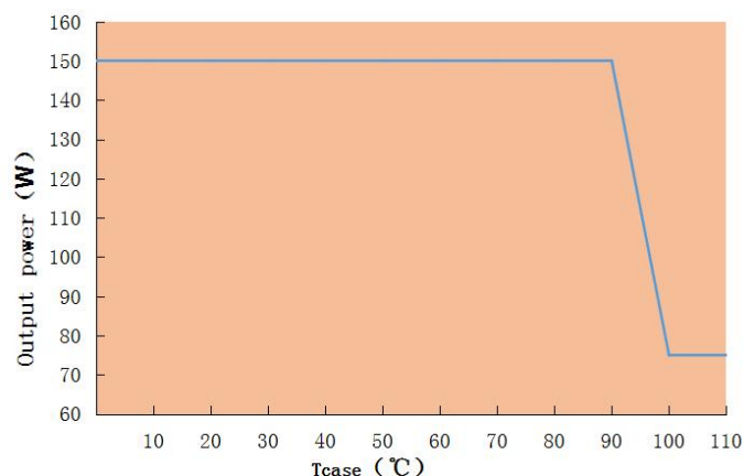
Output power VS Tcase(HVC-150W-56 & 214A/B/C)
