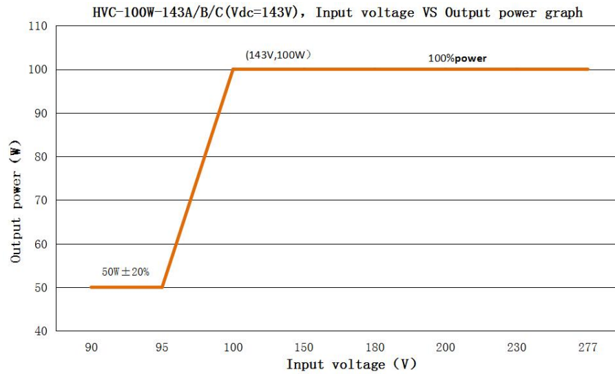
HVC-100W-143A/B/C (For output 143Vdc, the rated output current & power under different input voltage)
