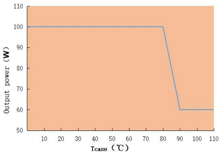
Output power VS Tcase(HVC-100W-56&143A/B/C)
