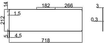
1: Reflective film requirement: Thickness: 0.3mm
