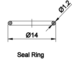
Seal Ring
