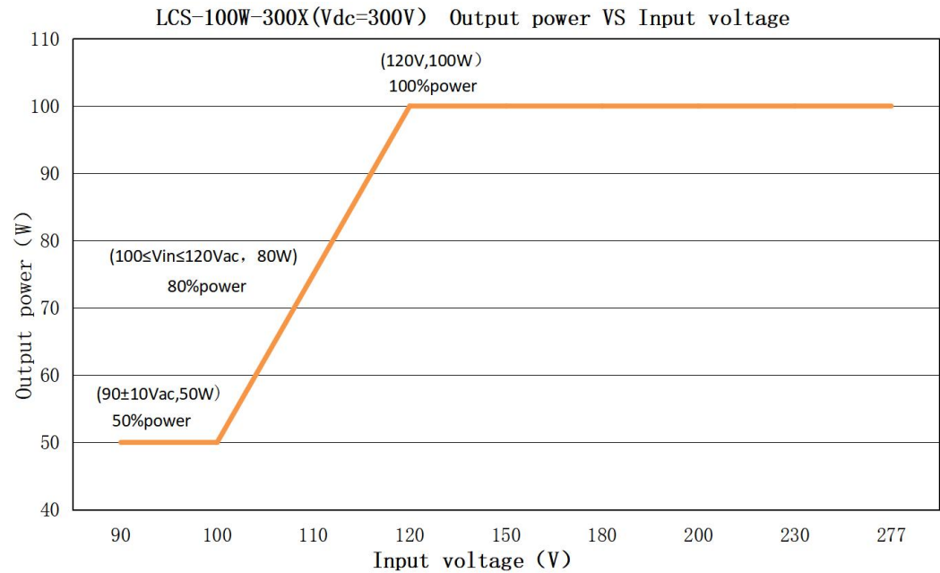
LCS-100W-300X(For output 300Vdc, the rated output current & power under different input voltage)
