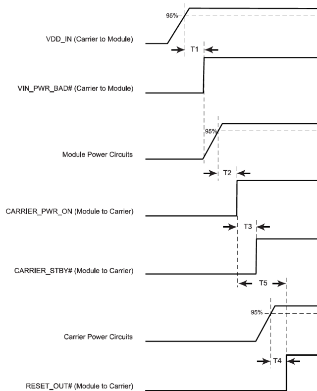
Figure 6: Power Input Sequencing
