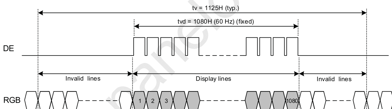
Fig. 9.2 Vertical Timing
