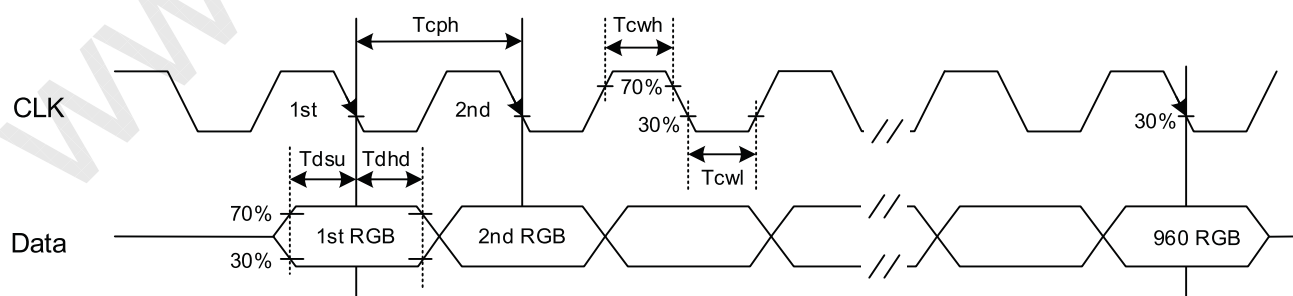
Fig. 9.3 Setup &amp; Hold Time
