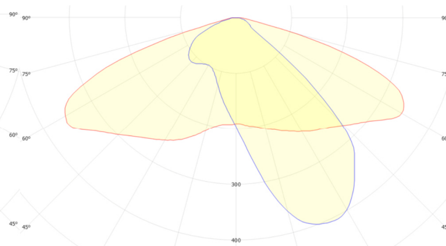
GSLED 5050.V6X.20 FWHM = 144°×48°, \eta = 93,0 %
