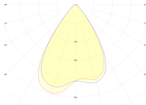
Samsung LH351C FWHM = 68°, \eta = 93,3 %
