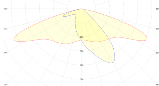
Refond RF-Q50SA40B FWHM = 146°×45°, \eta = 96,3 %
