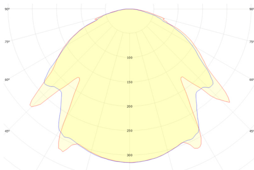
GSLED 5050.V6X.20 FWHM = 118° × 117°, η = 93,9 %
