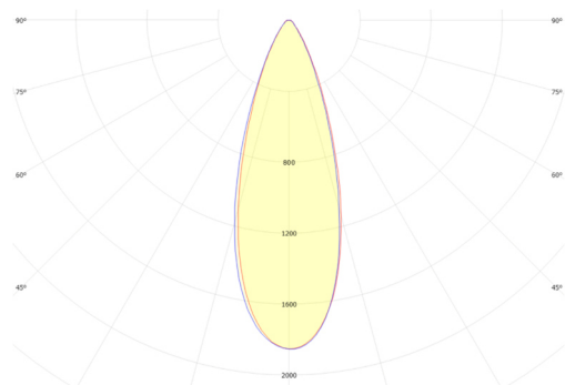
GSLED 5050.V6B.50 FWHM = 35°, \eta = 90,1 %
