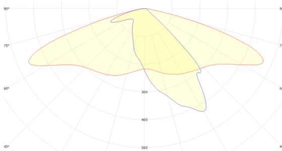
GSLED 5050.V6B.50 FWHM = 147°×46°, \eta = 93,5 %
