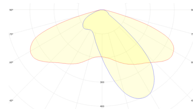
Refond RF-Q50SA40B FWHM = 145°×47°, \eta = 93,3 %
