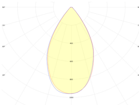
GSLED 5050.V6X.40 FWHM = 60°, \eta = 92,0 %
