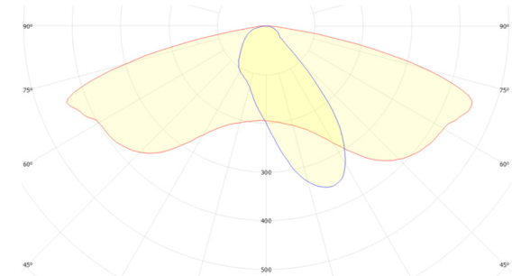
Refond RF-Q50SA40B FWHM = 155°×44°, \eta = 94,8 %
