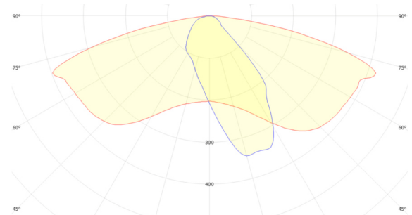
GSLED 5050.V6B.50 FWHM = 157°×46°, \eta = 92,4 %
