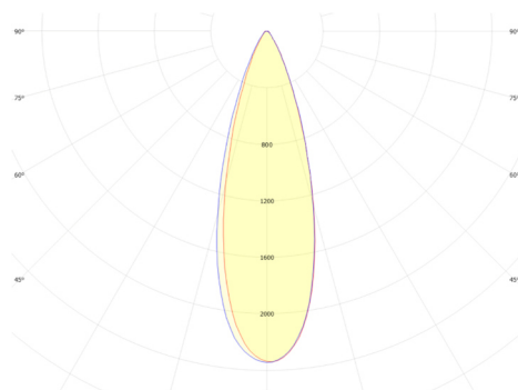
GSLED 5050.V6X.20 FWHM = 31°, \eta = 91,0 %
