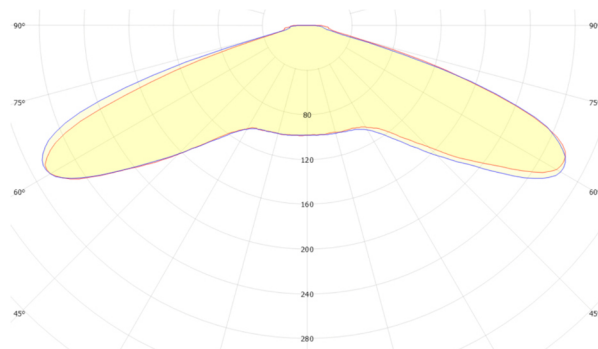
GSLED 5050.V6X.20 FWHM = 143°×144°, \eta = 93,4 %
