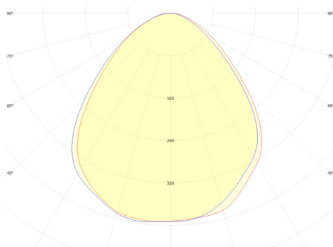
GSLED 5050.V6B.50 FWHM = 92°, \eta = 87,8 %
