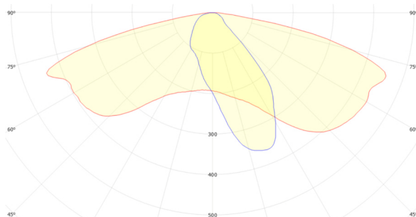
GSLED 5050.V6X.40 FWHM = 156°×44°, \eta = 94,8 %
