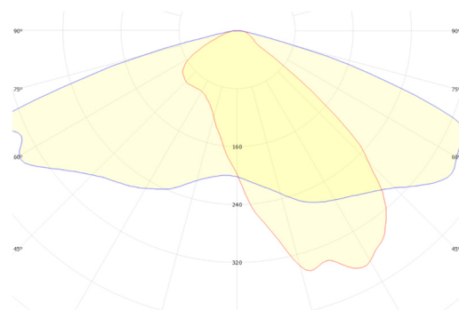
GSLED 5050.V6X.20 FWHM = 147°×51°, \eta = 91,1 %
