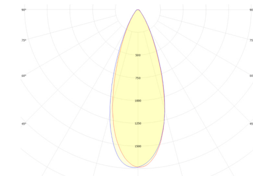
OSRAM DURIS S8 FWHM = 36°, \eta = 91,0 %
