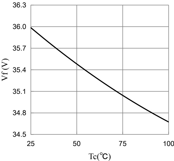
Case Temperature vs. Forward Voltage ( I_f=480\text{mA} )
