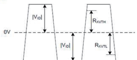
LVDS DC Diagram
