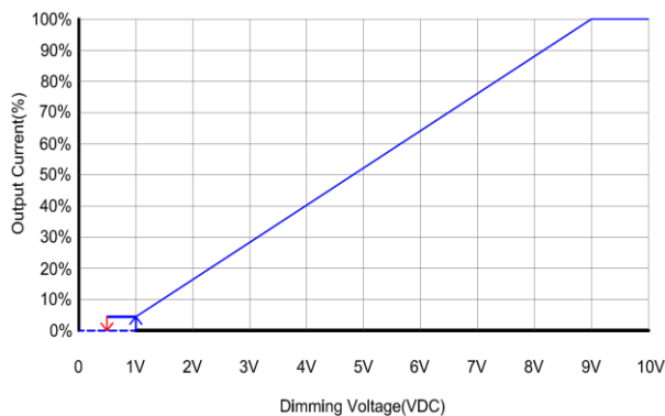
Dimming curve
