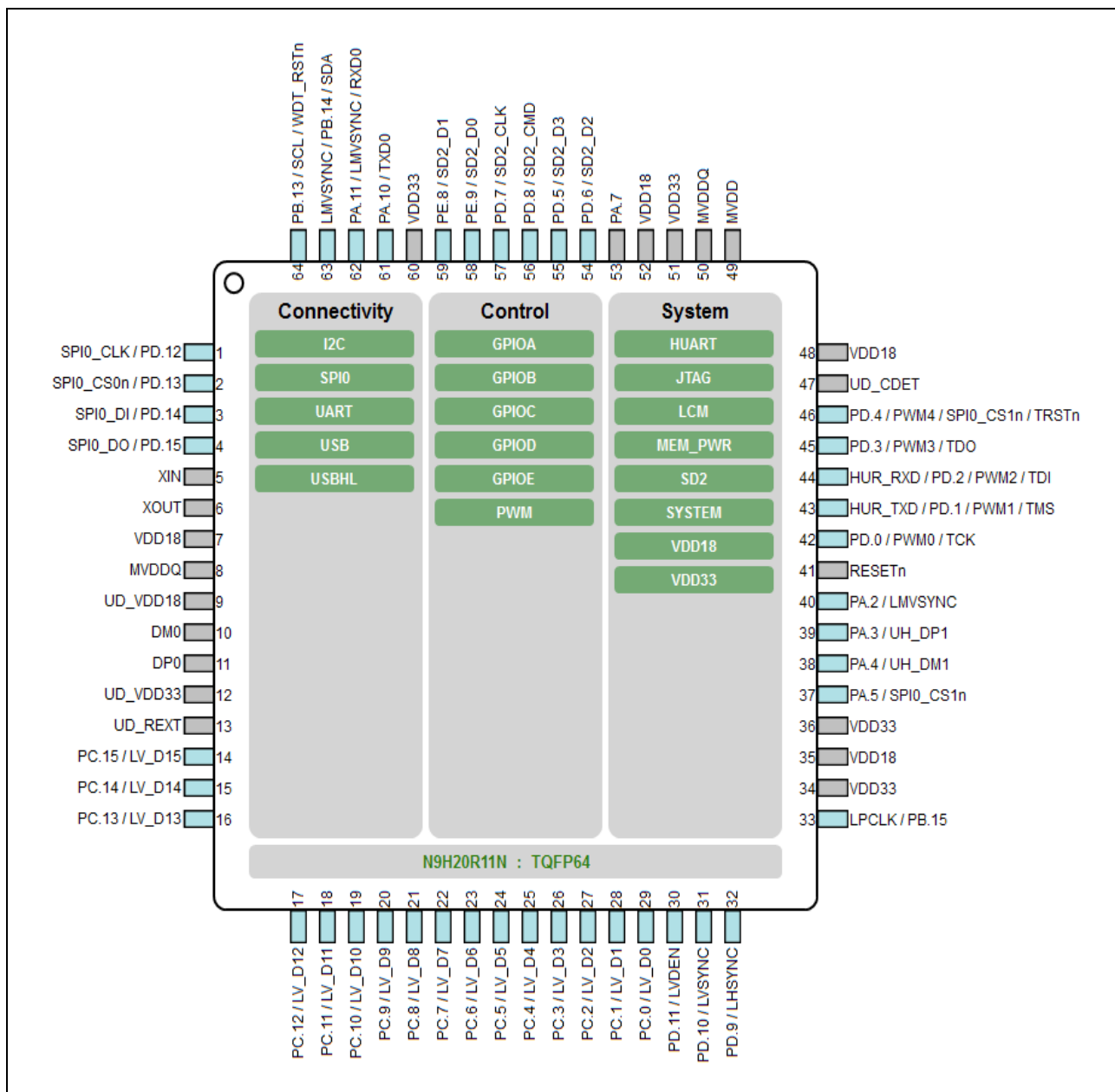
Figure 3.3-2 N9H20R11N TQFP 64 Pin Diagram
