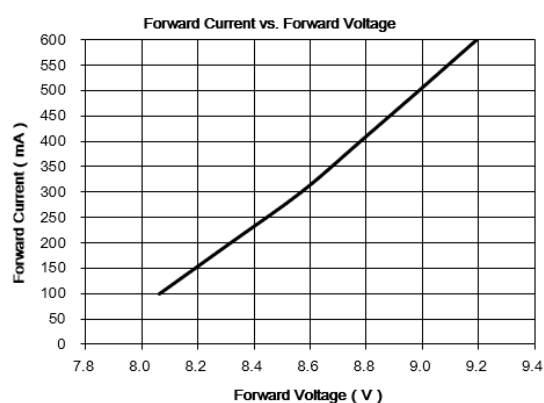
Forward Voltage Vs. Forward Current 伏安特性曲线
