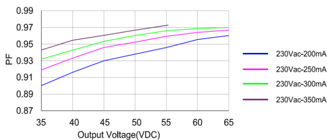
Power Factor Characteristics
