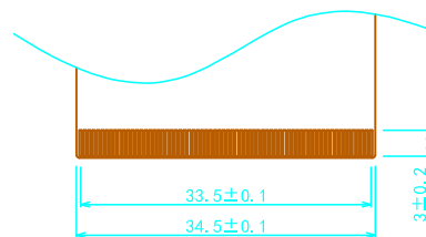
DETAIL A SC 4:1
