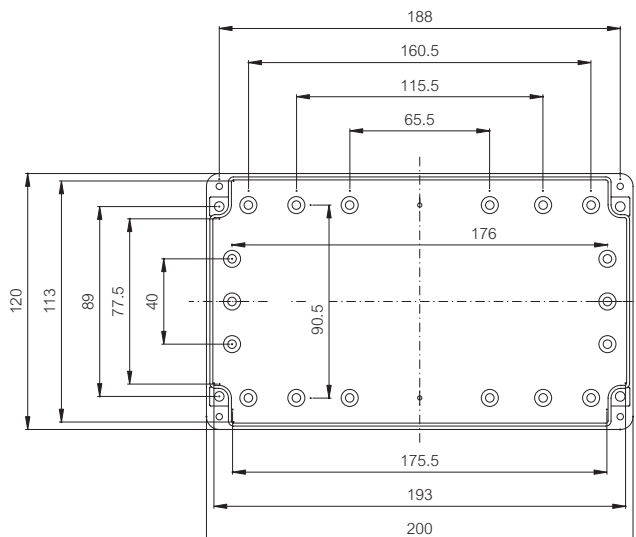
EURONORD PC/ABS 200x120x75-90
