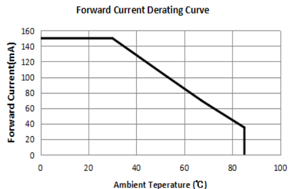
Ambient Temperature VS Allowable Forward Current 环境温度与允许温度电流特性
