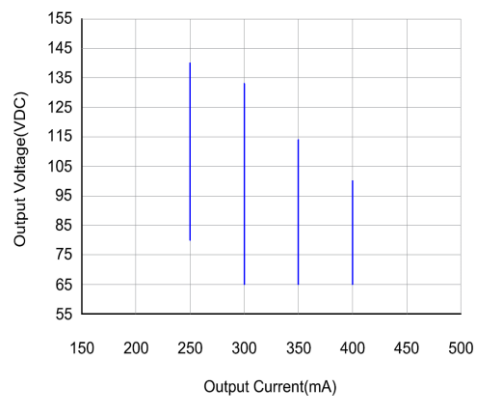
Operating window
